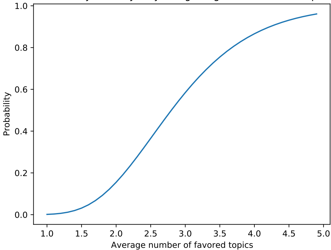
Probability of everybody being assigned a favorable topic
