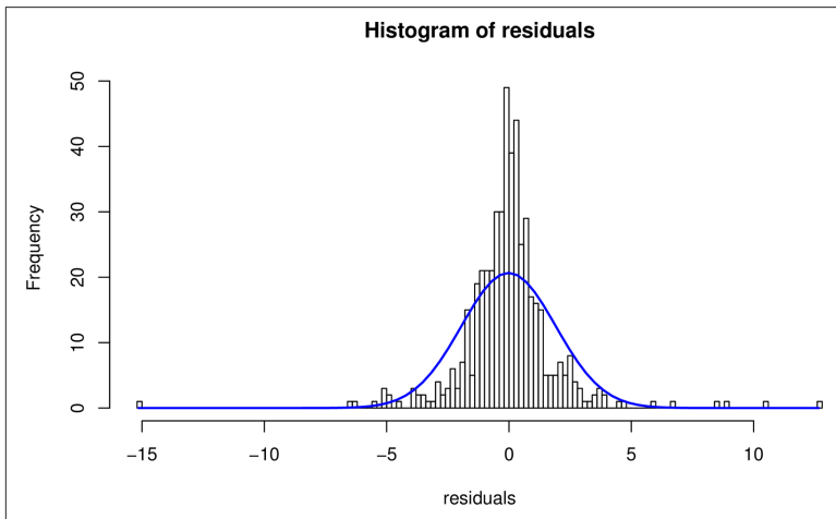
Figure 5-1. Histogram of residuals from the control chart on differenced data.
